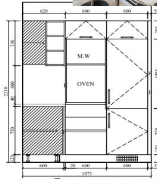
③ ELEVATION 2
